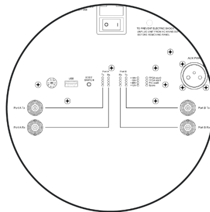
16: CDC I/O 6448 - 2 pairs of MegaCOMMS ports
